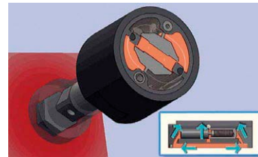
Fully opened relief valve when pulsing.
